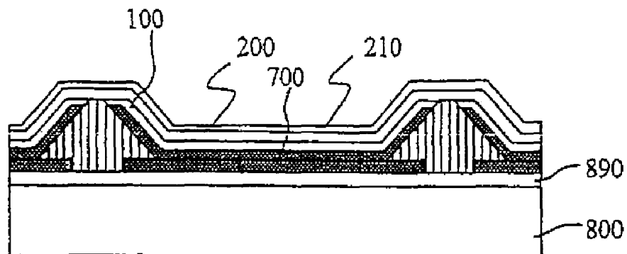
FIG.25B EXPOSURE
